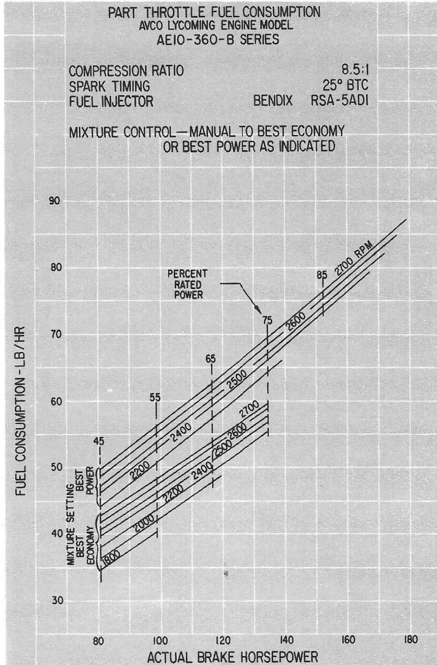
Figure 4-7. Part Throttle Fuel Consumption - AEIO-360-B, -H Series
